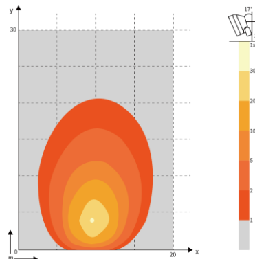
30W 3000lm
