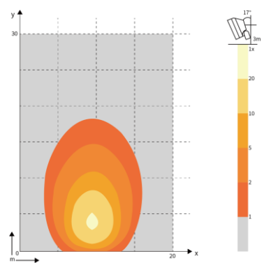
18W 2200lm
